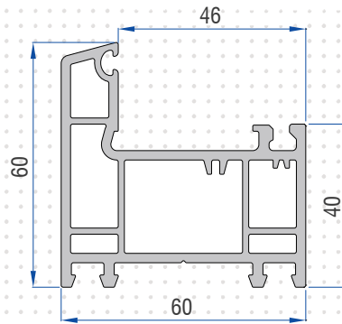
Frame Profile 77601 - 10210
