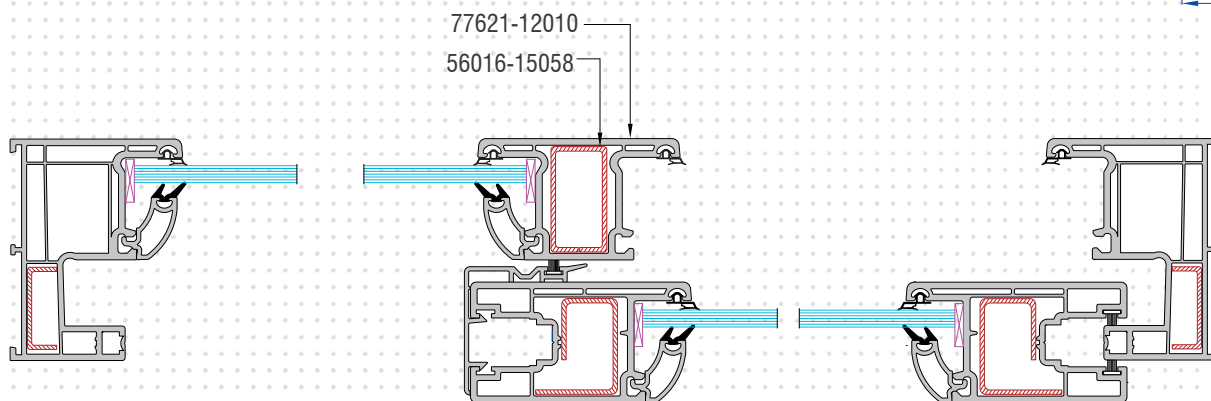
Sec B-B
