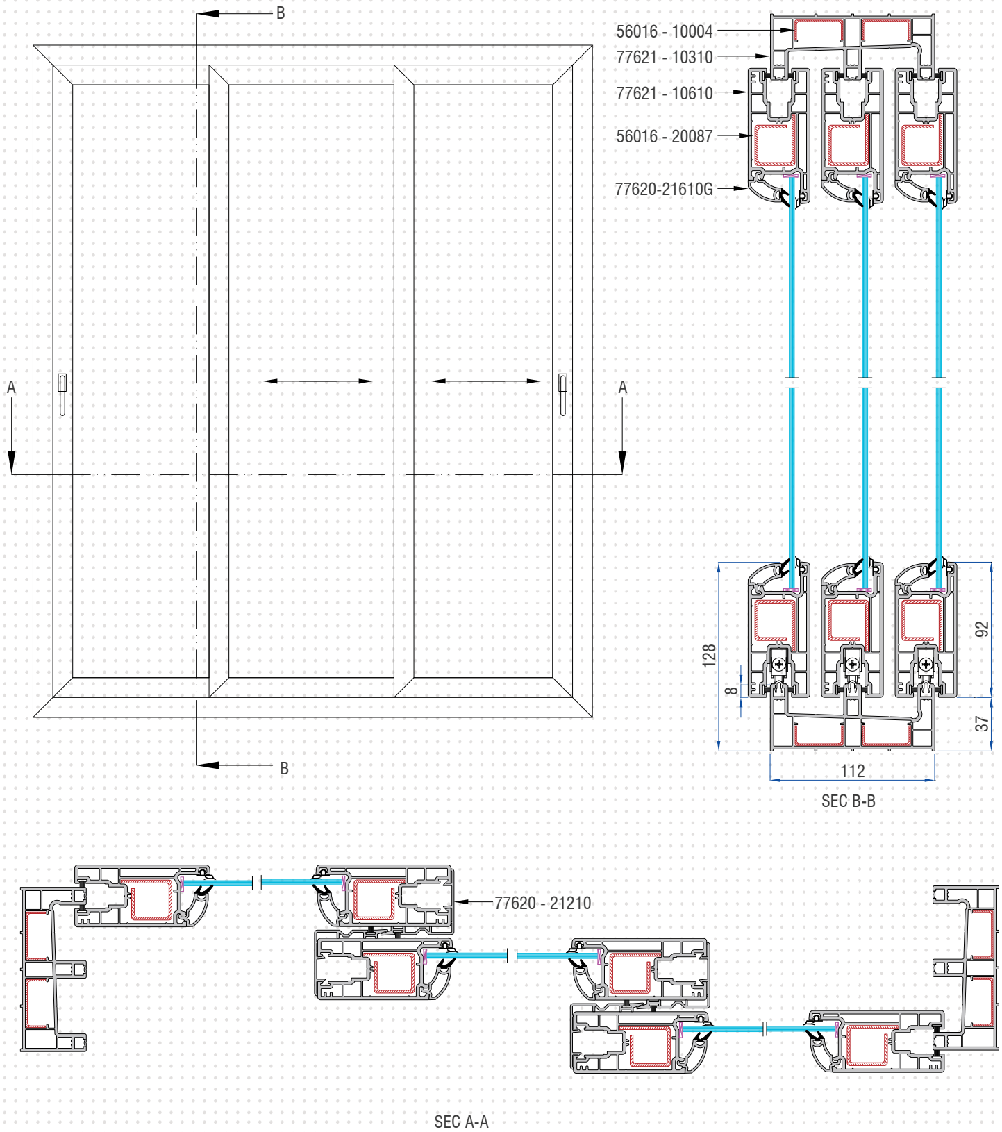
3 TRACK 3 PANEL DOOR
