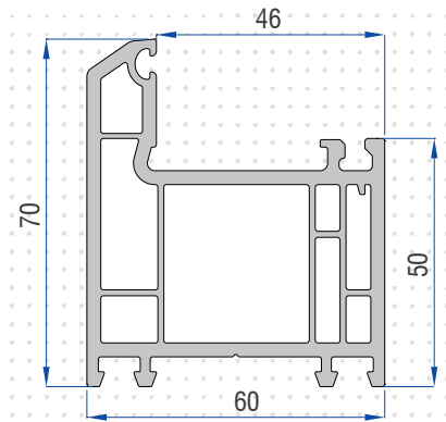
Large Frame Profile 77601 - 11910
