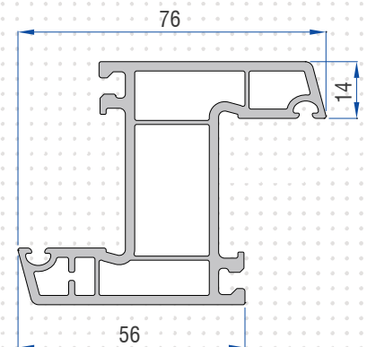
Z-Mullion Profile 77601 - 10610
