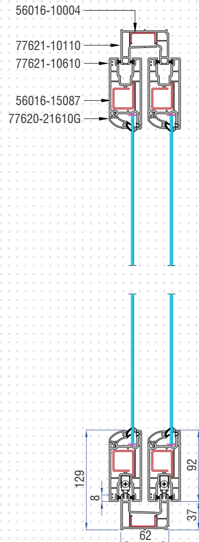
SEC B-B
