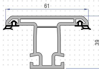
Sash/Mullion profile 77391-10210
