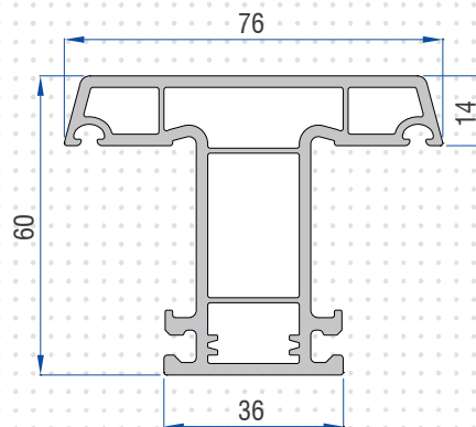
T-Mullion Profile 77601 - 10510
