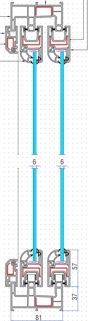
SEC B-B
