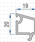
Double Glazing Bead 77600 - 21010
