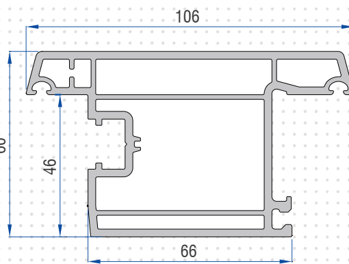
Outward Door Sash Profile 77601 - 10410
