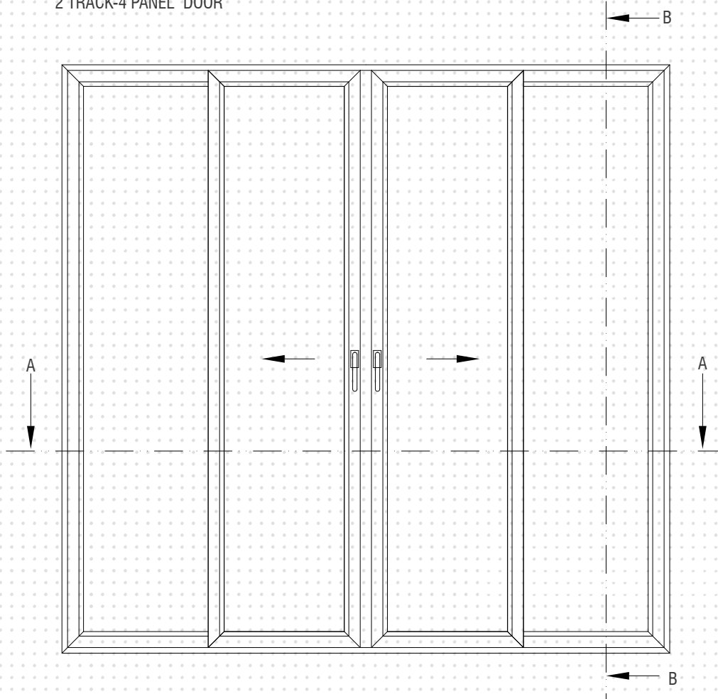
2 TRACK-4 PANEL DOOR
