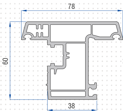
Outward Window Sash Profile 77601 - 10310
