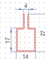
Sash/ Mullion Reinforcement 56012-08051
