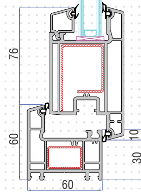
SEC B-B
