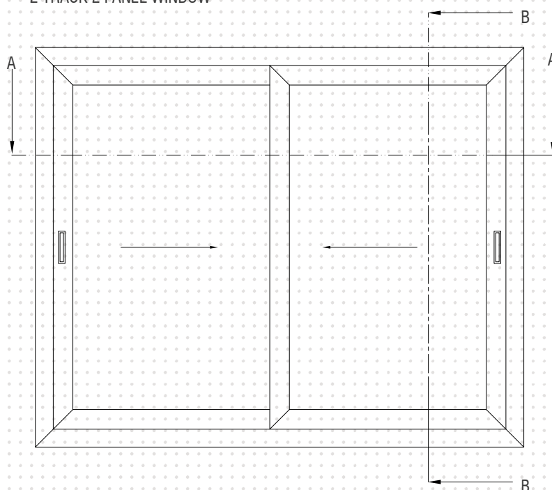
2 TRACK 2 PANEL WINDOW
