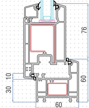
SEC B-B
