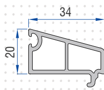
Single Glazing Bead 77600 - 20910
