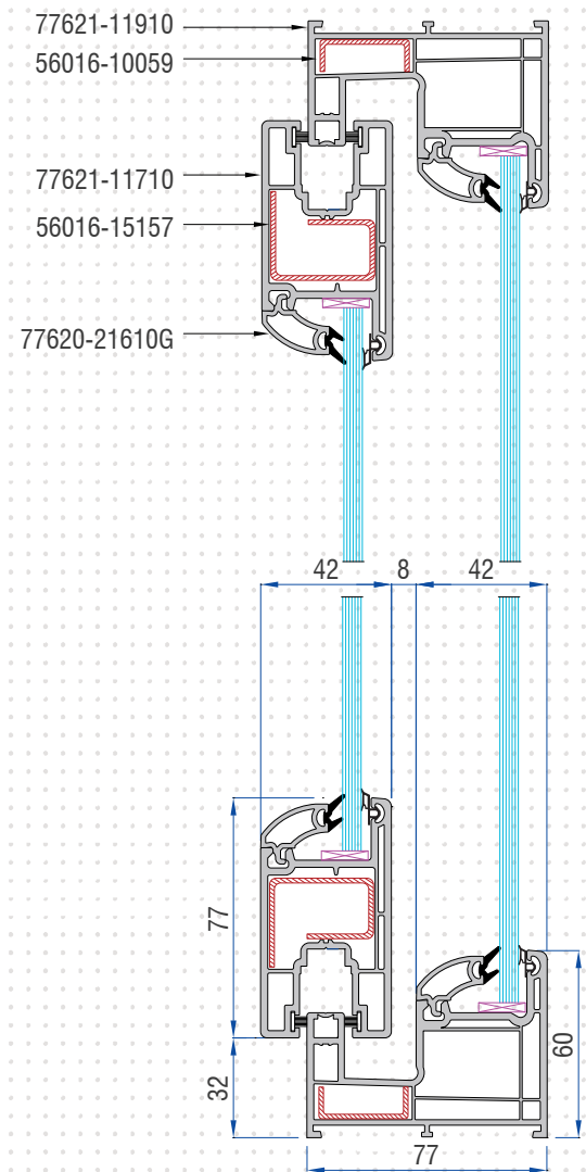
Sec B-B
